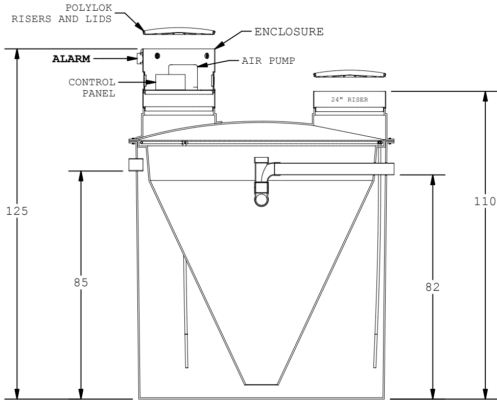
AERATION TANK
