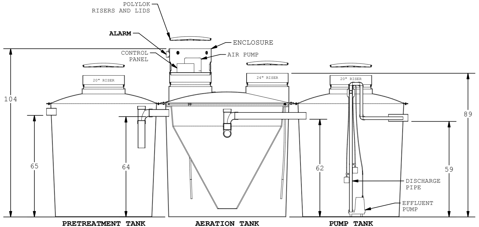
PRETREATMENT TANK
