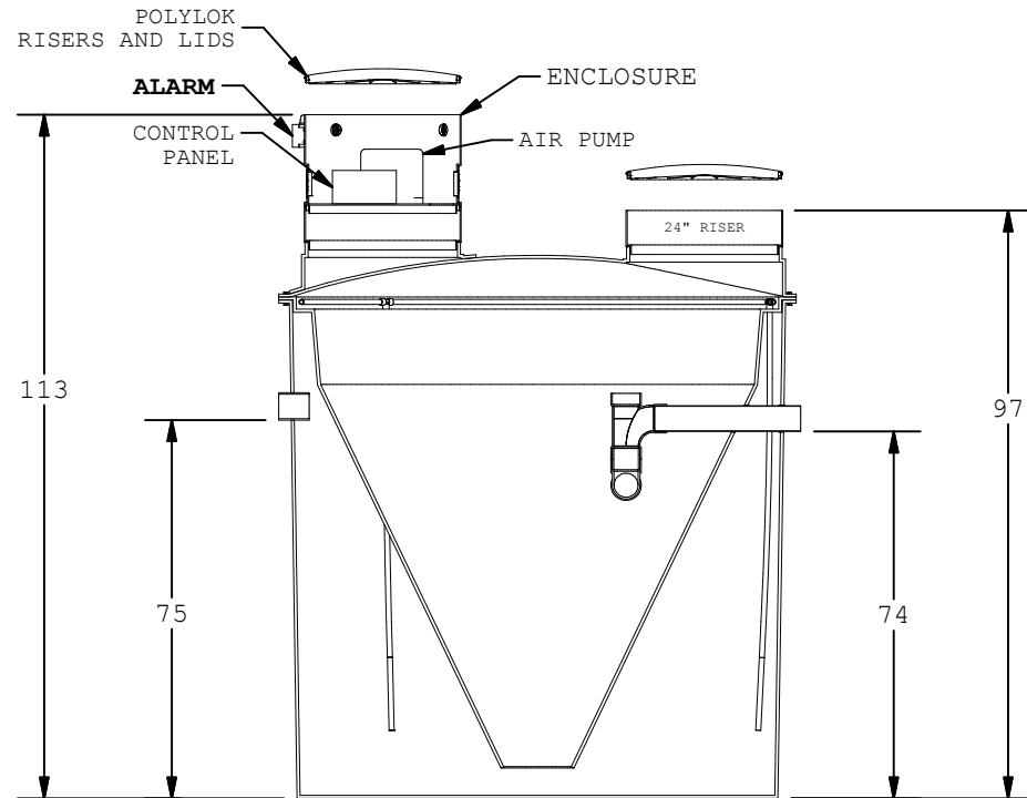
AERATION TANK
