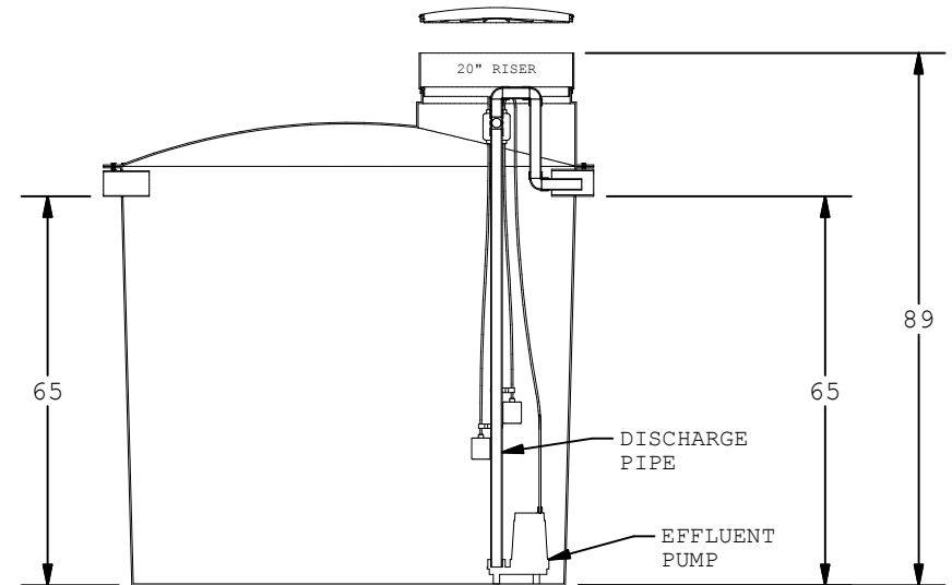
PUMP TANK
