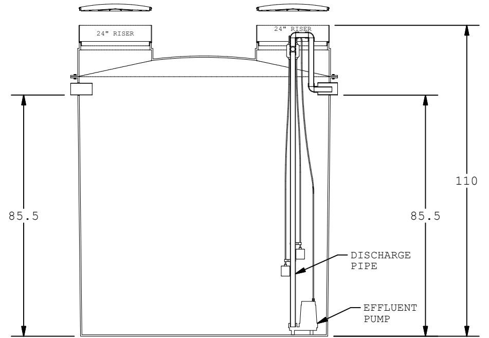
PUMP TANK
