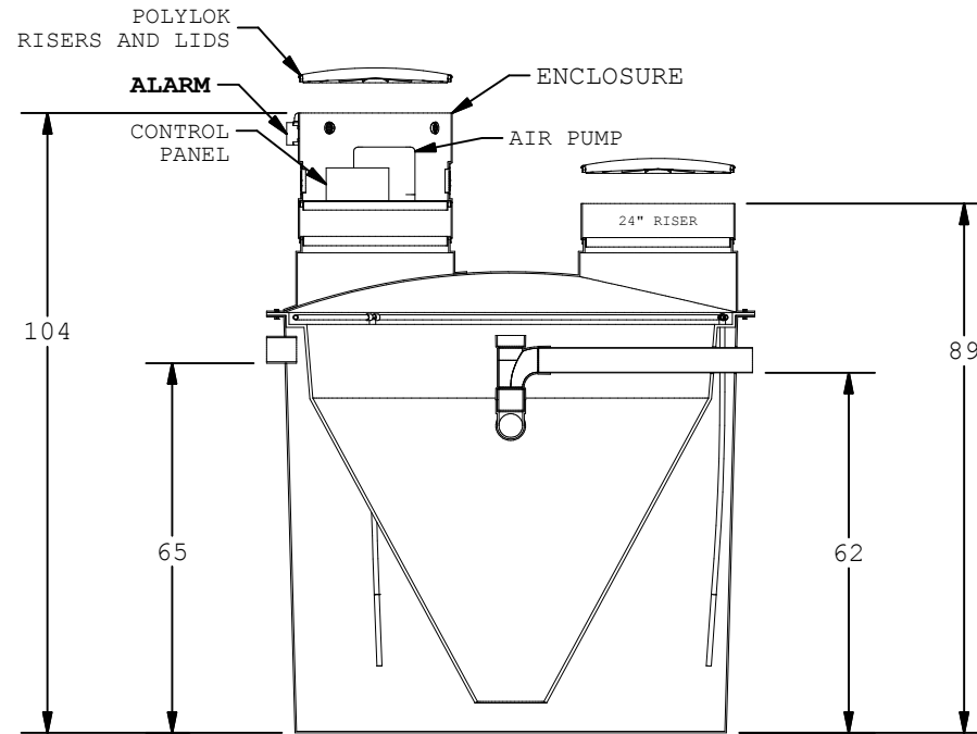
AERATION TANK
