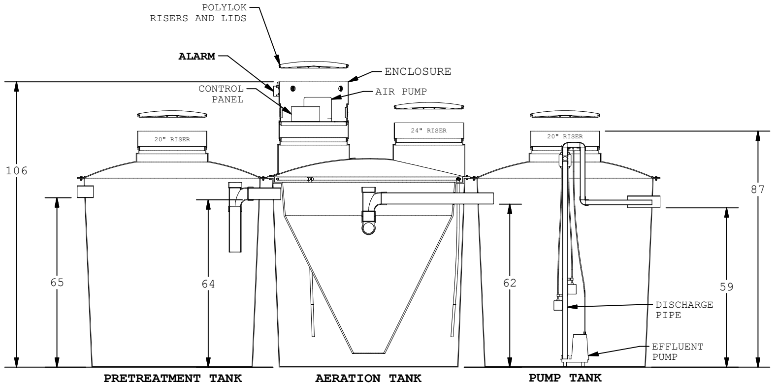
PRETREATMENT TANK
