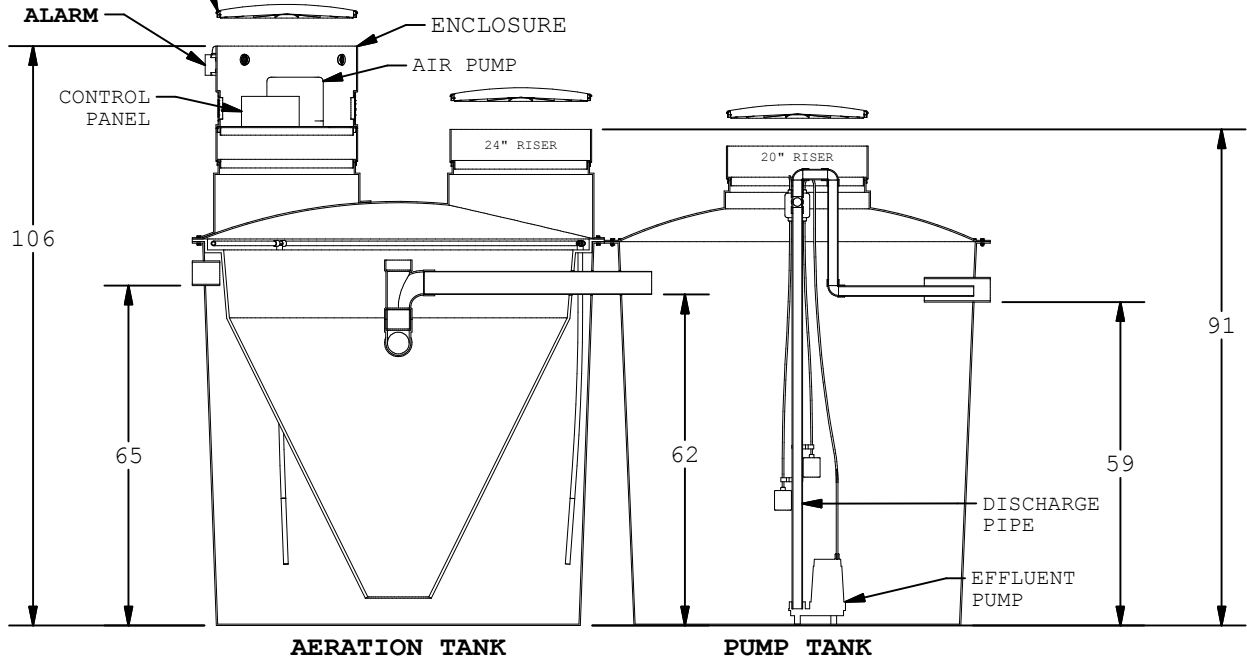
AERATION TANK
